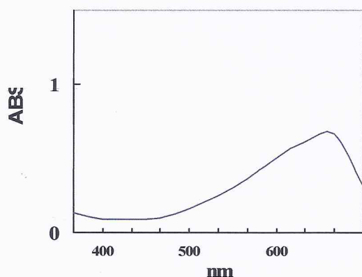
Spectral reflectance
